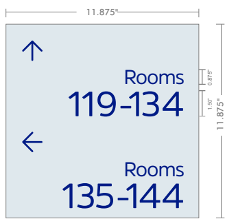
2-LINE ROOM DIRECTIONAL HDX-1102
