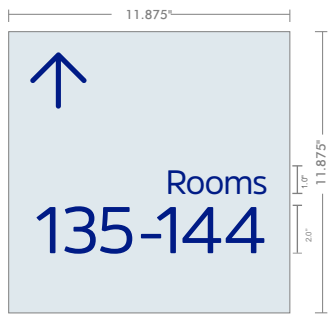
ROOM DIRECTIONAL HDX-1101
