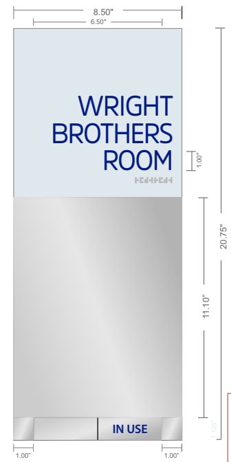
MEETING ROOM HDX-1529
